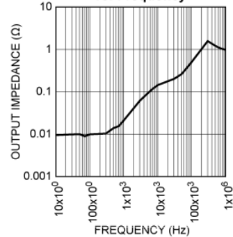
MIC2975x Output Impedance vs. Frequency
