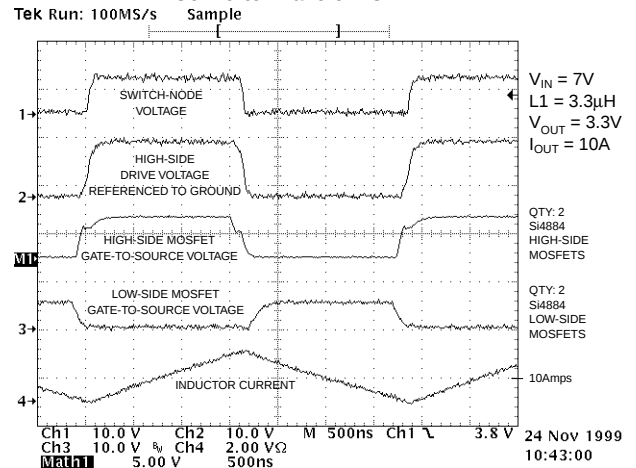
Converter Waveforms
