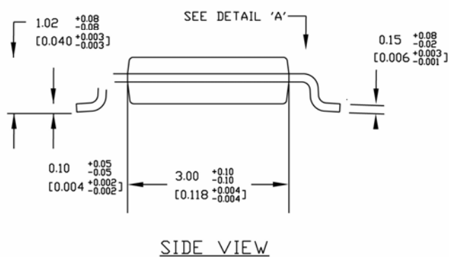
10-Pin MSOP (MM)
