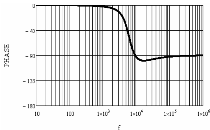
Figure 9. Phase Curve for G(s)
