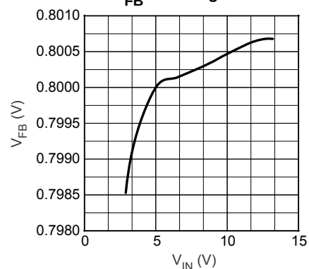
V_{FB} Line Regulation
