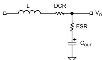
Figure 7. The Output LC Filter in a Voltage-Mode Buck Converter
