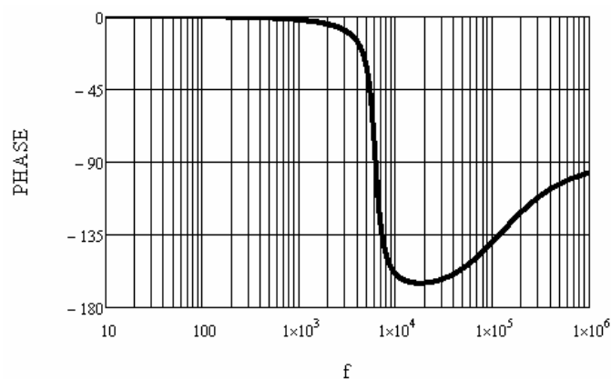
Figure 10. The Phase Curve with ESR = 0.002Ω
