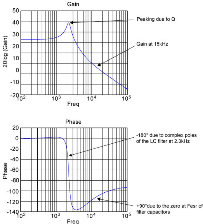
Figure 12. Modulator Transfer Function
