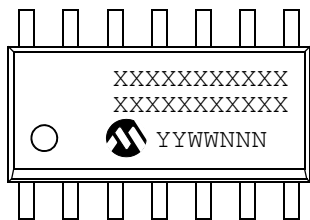
14-Lead SOIC (150 mil) (MCP6S24)
