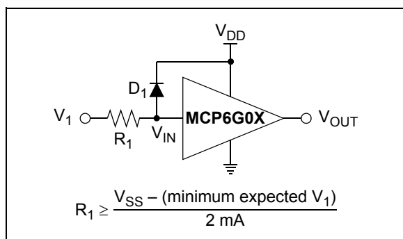
FIGURE 4-3: Protecting the Analog Inputs.
