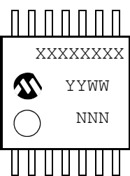
14-Lead TSSOP (4.4mm) (MCP6S24)
