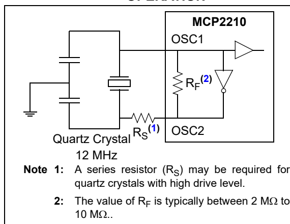
FIGURE 1-5: QUARTZ CRYSTAL OPERATION
