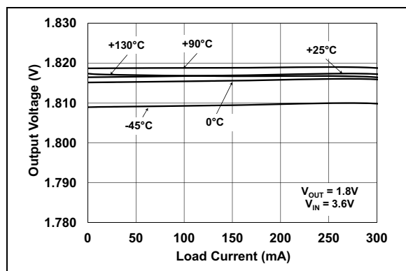
FIGURE 2-9: Output Voltage vs. Load Current.
