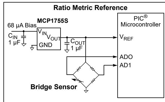
FIGURE 5-2: Using the MCP1755/MCP1755S as a Voltage Reference.
