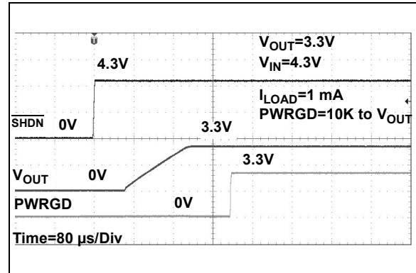
FIGURE 2-28: Start-up from \overline{\text{SHDN}} .
