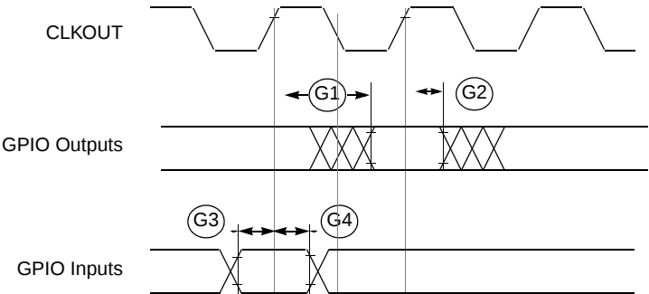
Figure 16. GPIO Timing
