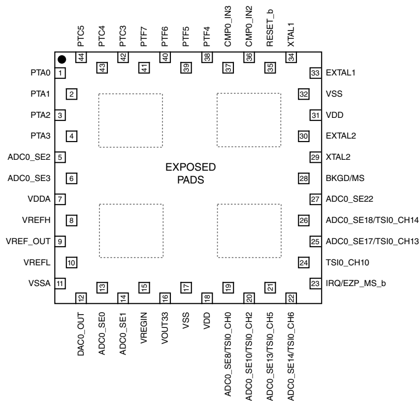
Figure 20. 44-pin Lamine QFN
