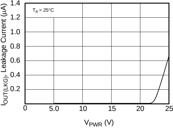
Figure 20. Sleep State Output Leakage vs. V_{PWR}
