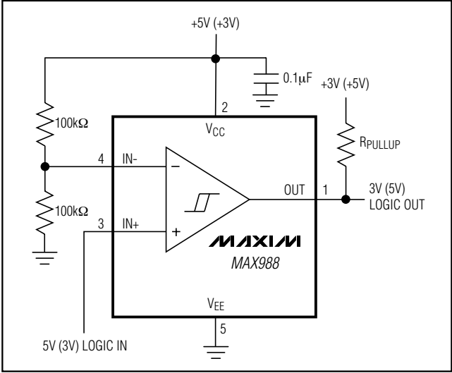
Figure 4. Logic-Level Translator
