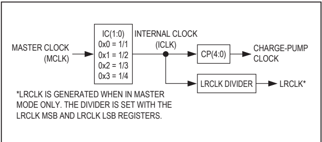
Figure 3. Internally Generated Clock Signals Derived from MCLK
