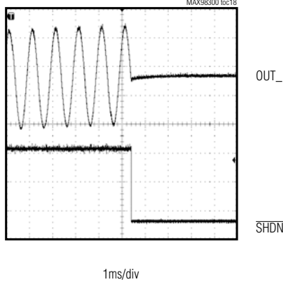
SHUTDOWN WAVEFORM
