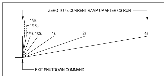
Figure 4. Ramp-Up Behavior
