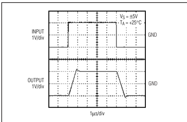
Figure 7b. Driving a 0.015μF Load with a 10Ω Isolation Resistor
