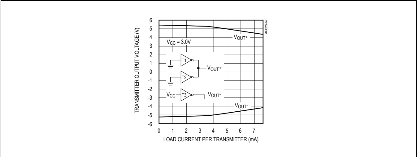
Figure 4a. MAX3241 Transmitter Output Voltage vs. Load Current per Transmitter
