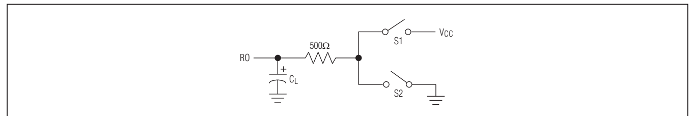
Figure 9. Receiver Enable and Disable Times
