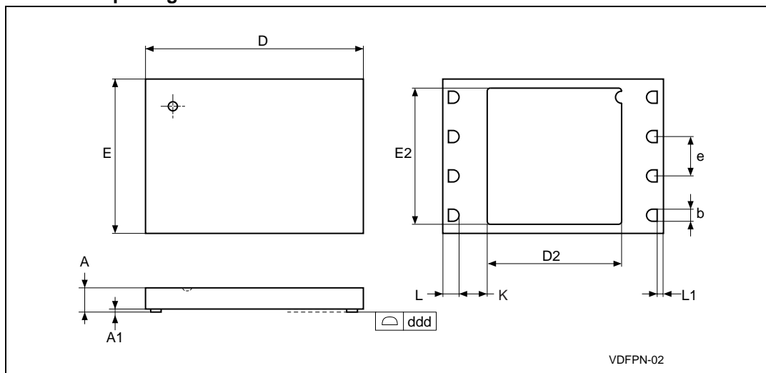
Figure 28. VDFPN8 (MLP8) 8-lead Very thin Dual Flat Package No lead, 8 x 6 mm, package outline
