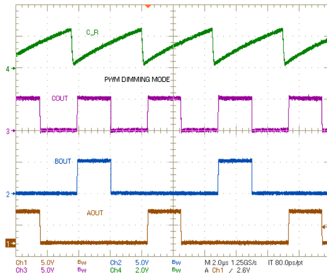
Figure 13 Channel 1: AOUT, Channel 2: BOUT Channel 3: COUT, Channel 4: C_R
