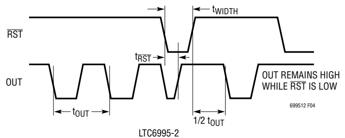
Figure 4. Reset Timing Diagram (POL Bit = 1)
