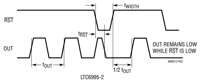
Figure 3. Reset Timing Diagram (POL Bit = 0)
