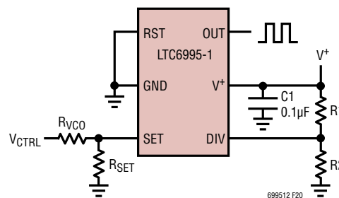
Figure 20. Voltage-Controlled Oscillator
