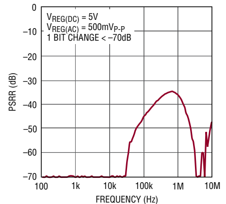
Measurement Error V_{\text{REG}} PSRR vs Frequency
