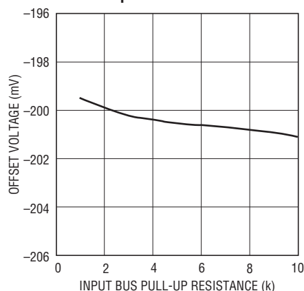
Input-Output Offset Voltage vs Pull-Up Resistance
