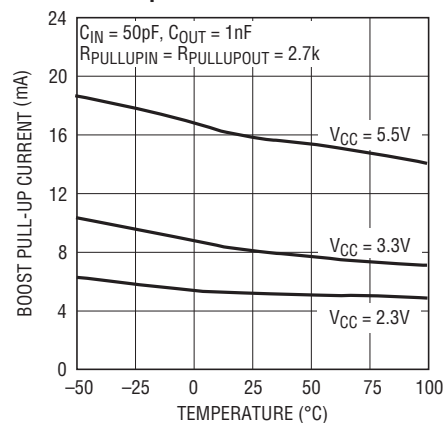
Boost Pull-Up Current vs Temperature
