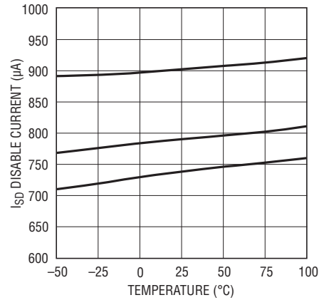
I_{SD} Disabled Current vs Temperature
