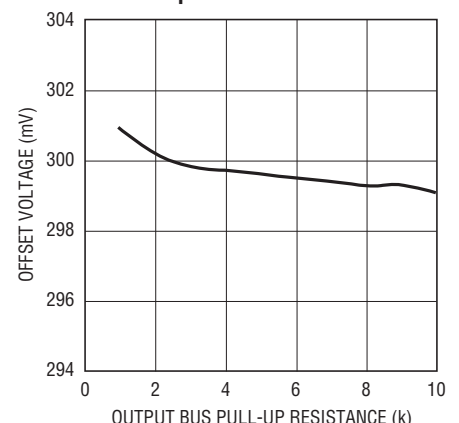
Output-Input Offset Voltage vs Pull-Up Resistance
