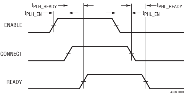
Rising and Falling Propagation Delays and Rise and Fall Times for SDAIN, SDAOUT and SCLIN, SCLOUT
