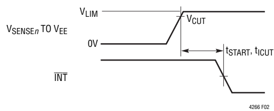
Figure 2. Current Limit Timing
