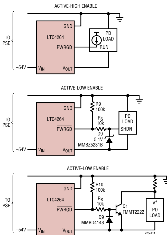
Figure 11. Power Good Interface Examples
