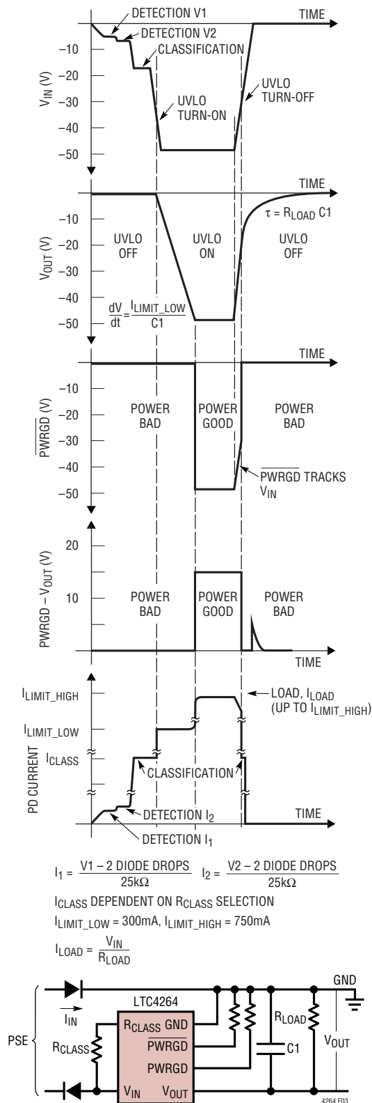
Figure 3. Output Voltage, \overline{\text{PWRGD}} , \overline{\text{PWRGD}} and PD Current as a Function of Input Voltage
