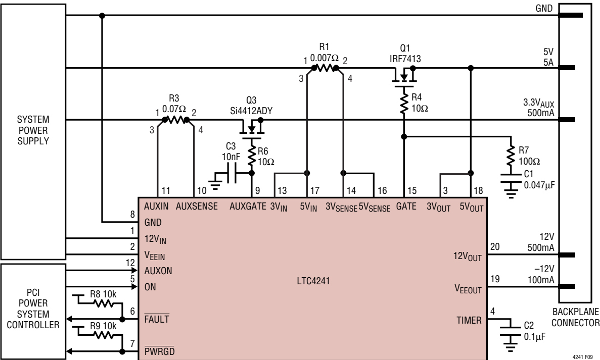
Figure 9. System Without 3.3V Supply
