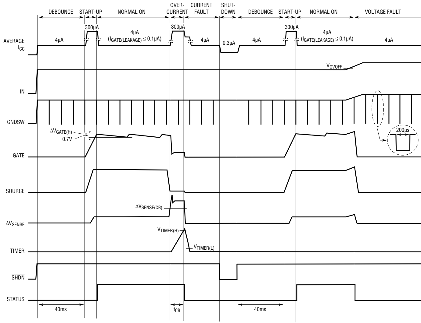
Figure 4. LTC4231-1 Overcurrent
