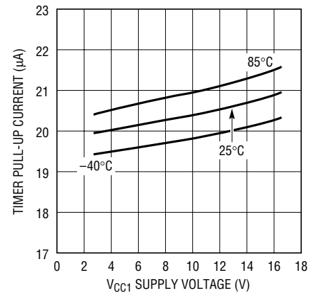
TIMER Pull-Up Current (During First Cycle) vs V_{\text{CC1}} Supply Voltage
