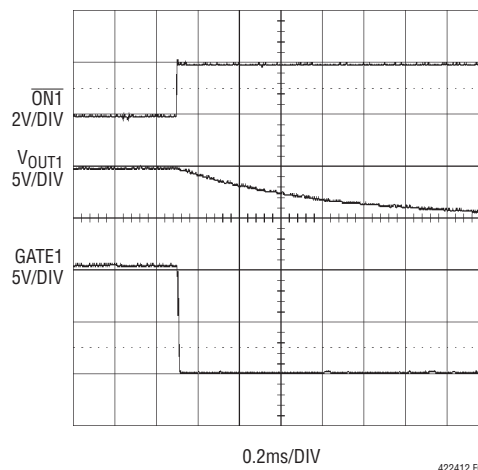
Figure 4. Normal Power-Down Sequence
