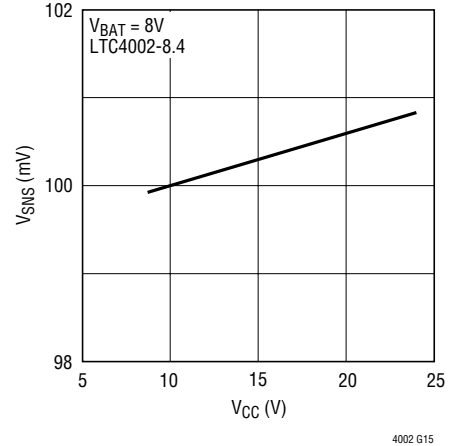
Current Mode Sense Voltage vs V_{CC}
