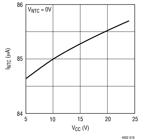
NTC Pin Output Current vs V_{CC}
