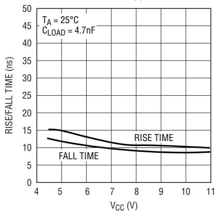
Rise/Fall Time vs V_{CC}
