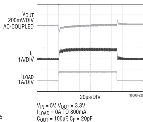
Load Step
