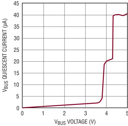
V BUS Current vs V BUS Voltage (Suspend)
