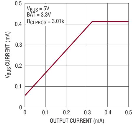
V BUS Current vs Output Current in Suspend
