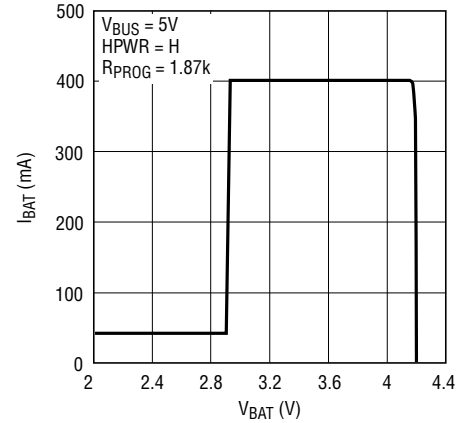
I BAT vs V BAT (LTC3554/LTC3554-2/LTC3554-3)
