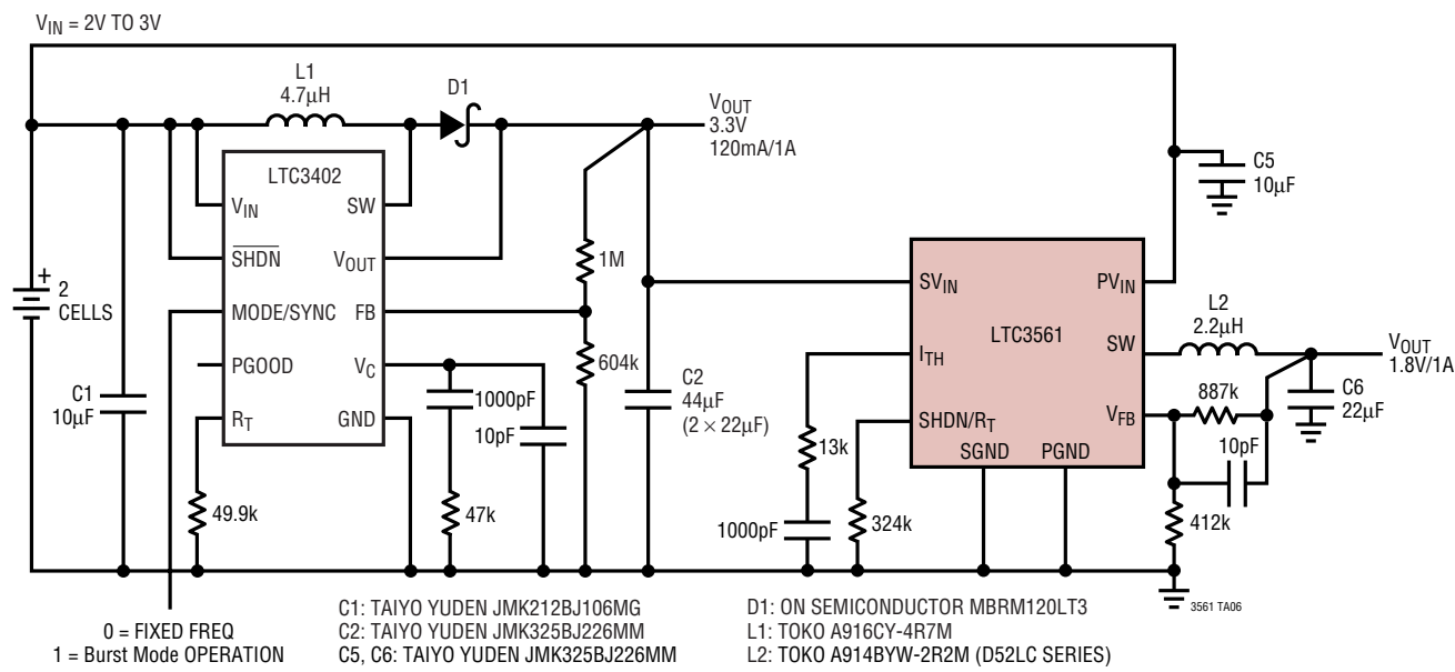
All Ceramic 2-Cell to 3.3V and 1.8V Converters
