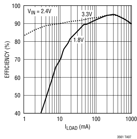
Efficiency and V_{OUT} Ripple
