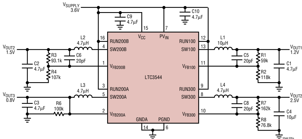
Figure 5. Design Example
