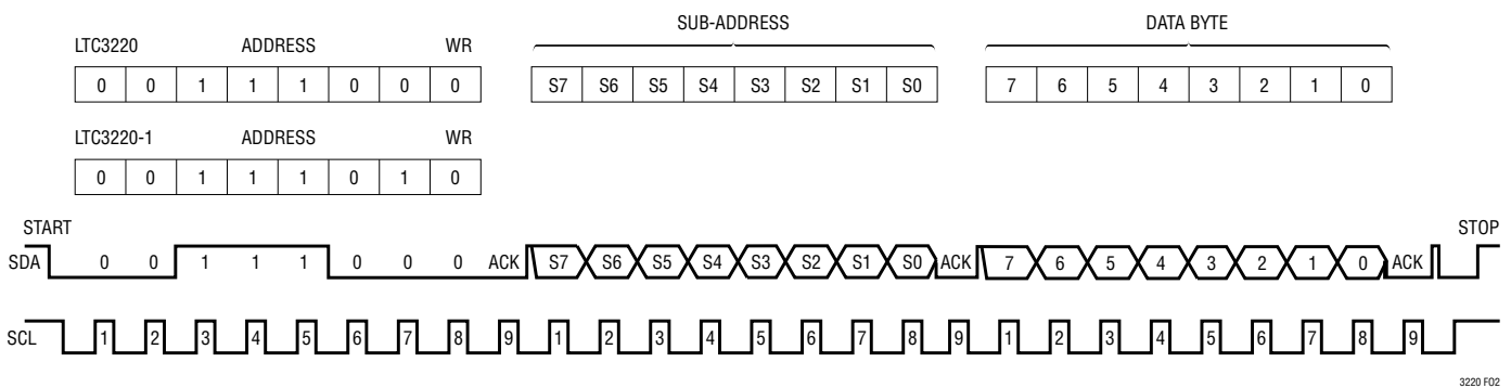
Figure 2. Bit Assignments
