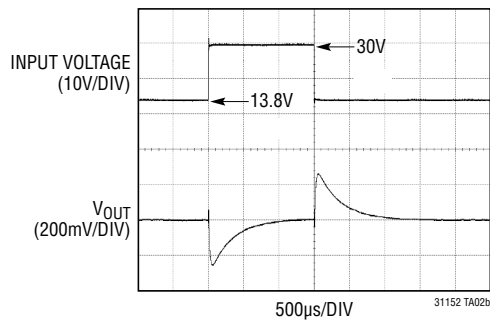
Fast (10 \mu s) Line Transient from V_{IN} = 13.8V to 30V
