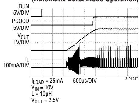
Start-Up from Shutdown (Automatic Burst Mode Operation)
