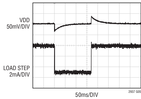
VDD Load Step Transient Response
