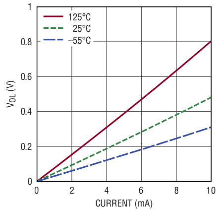
EN/\overline{n}V_{OL} vs Output Sink Current
