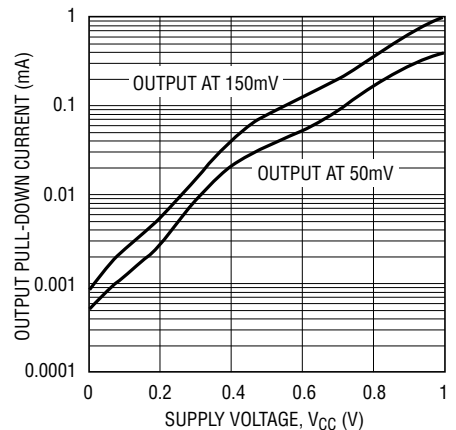
OUT1, OUT2, \overline{\text{RST}} Pull-Down Current vs V_{CC}
