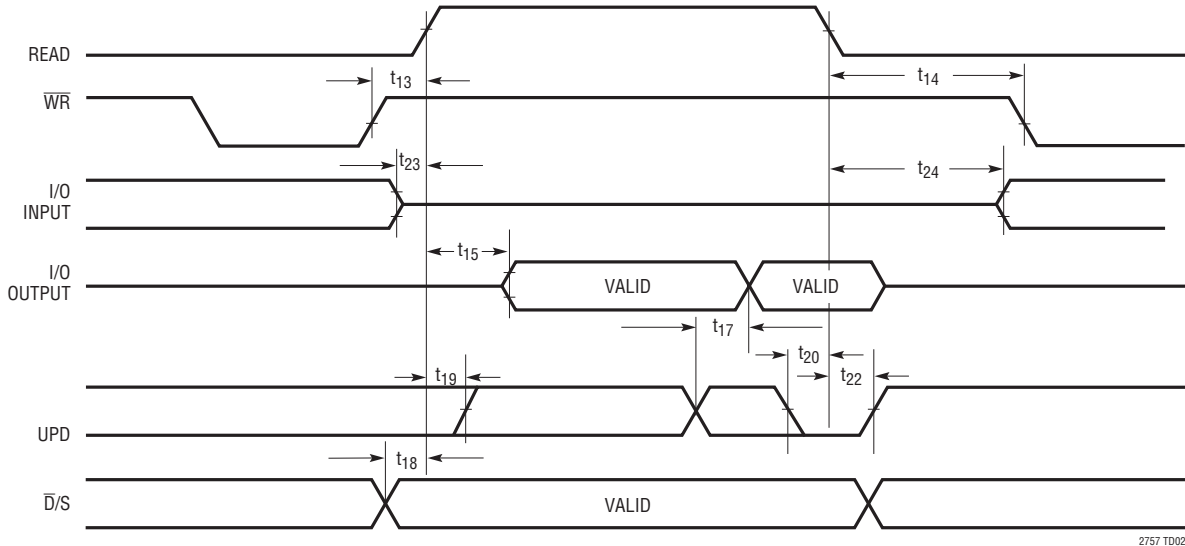
Readback Timing
