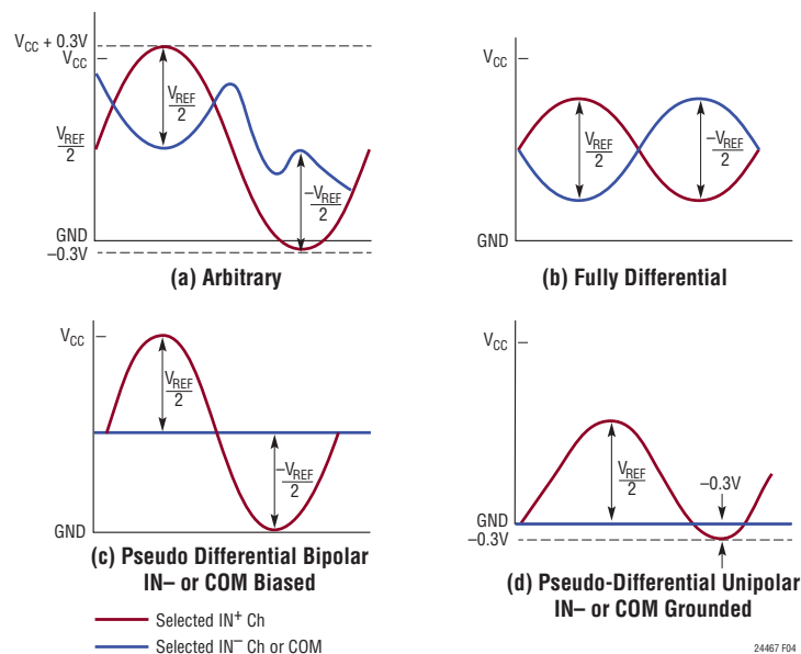
Figure 4. Input Range
