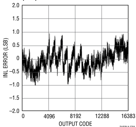
LTC2158-14: Integral Nonlinearity (INL)
