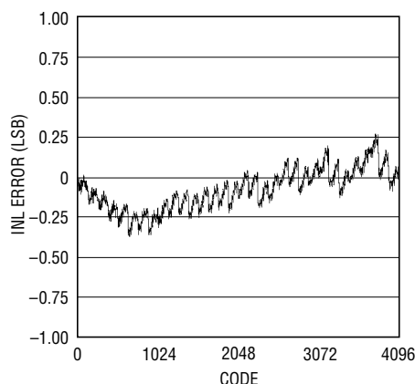
Typical INL
