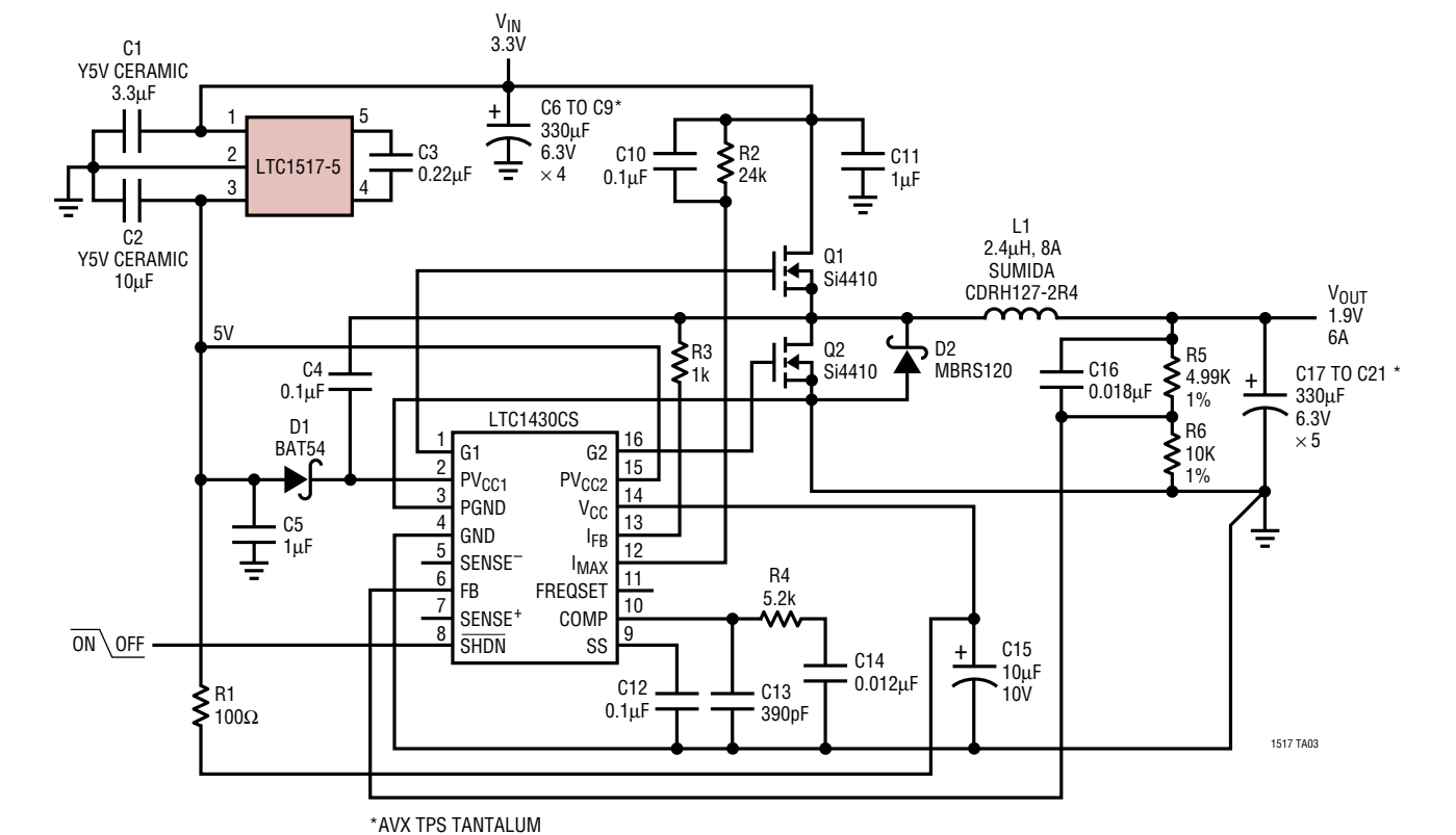
3.3V to 1.9V, 6A Power Supply
