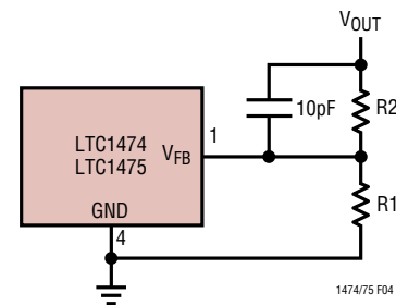
Figure 4. LTC1474/LTC1475 Adjustable Configuration
