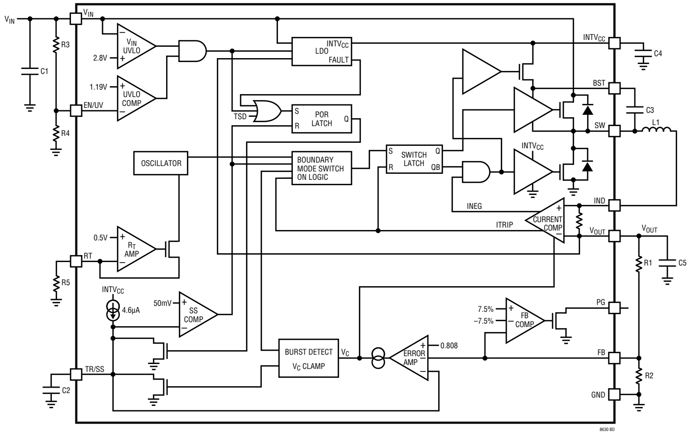
Figure 1. Block Diagram
