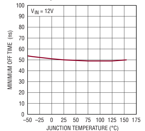
Switch Minimum Off-Time vs Temperature
