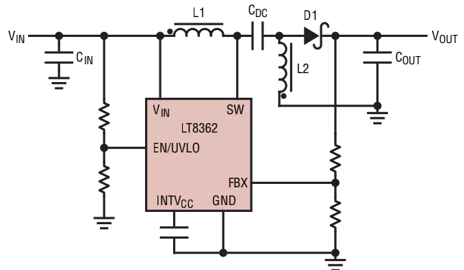
Figure 6. LT8362 Configured in a SEPIC Topology
