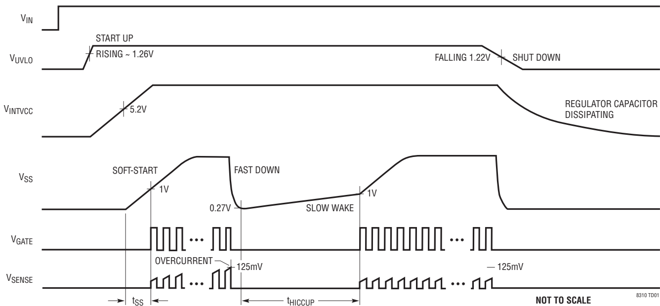
Start-Up/Soft-Start/Fault/Shutdown/Restart
