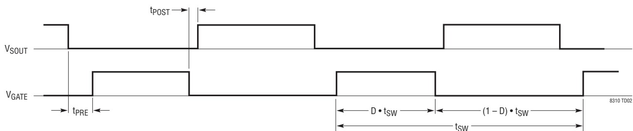
Nonoverlapping GATE/SOUT
