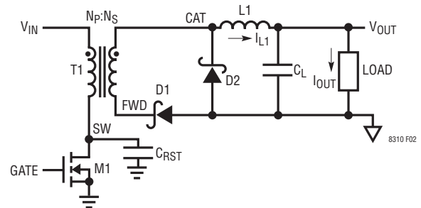
Figure 3. Forward Converter Architecture (Nonsynchronous)
