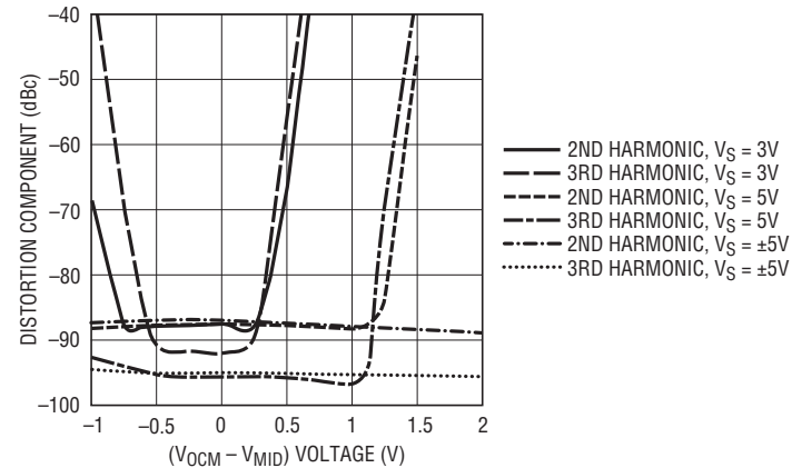
Distortion vs Output Common Mode Level, 2Vp-p 1MHz Input, 1x Gain, T_A = 25^\circ C
